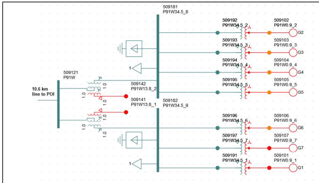
Figure A-1: Survey Mountain Wind Project Single Line Diagram for Power Flow Study.
