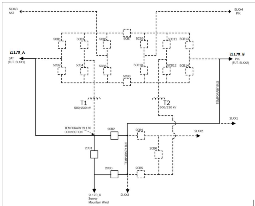
Figure C-1: Stations Planning Conceptual One-Line Sketch for the New Switching Station P77T After Potential Conversion to 500/230 kV Substation.
