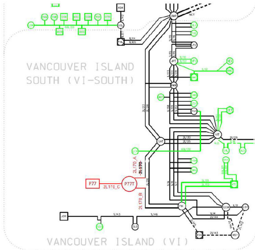
Figure 1-1: South VI 132/230 kV Transmission System Diagram in 2024 with the Proposed Survey Mountain Wind Project interconnection
