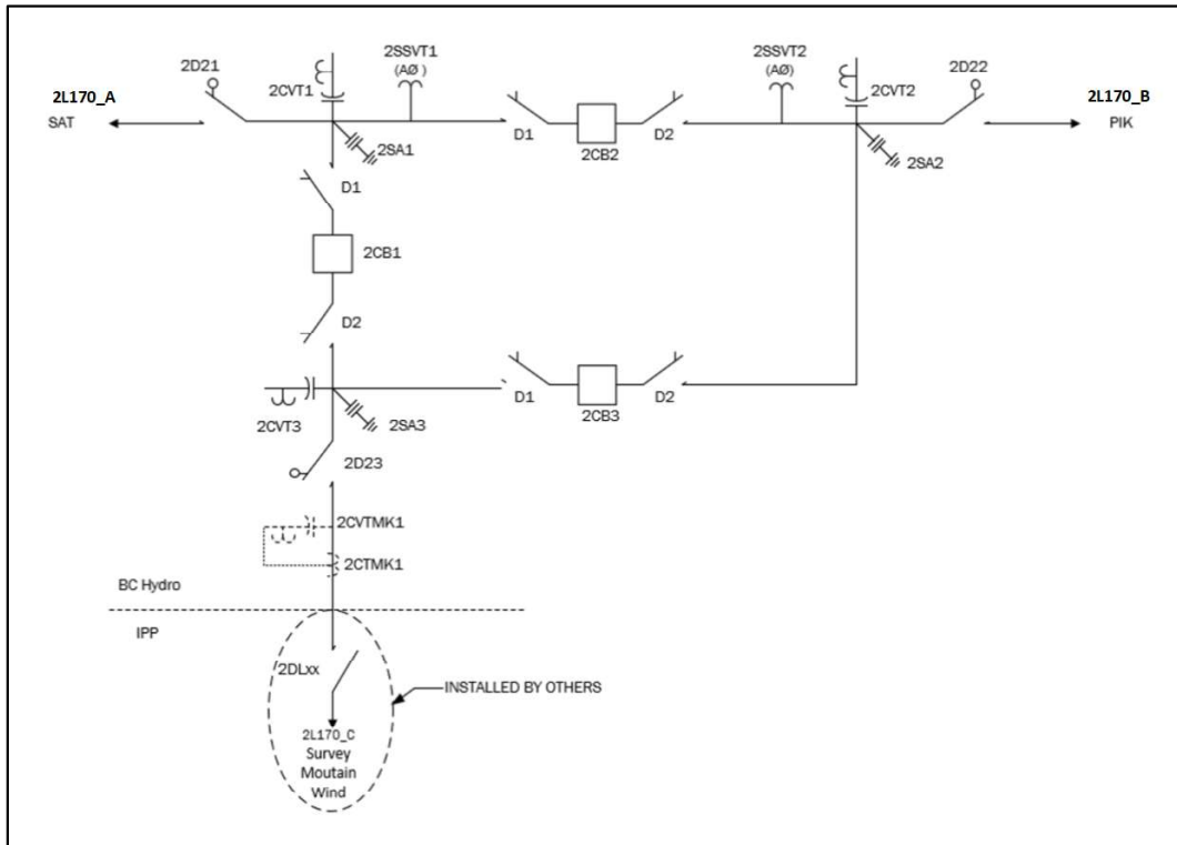
Figure B-1: Stations Planning One-Line Sketch for the New Switching Station P77T.
