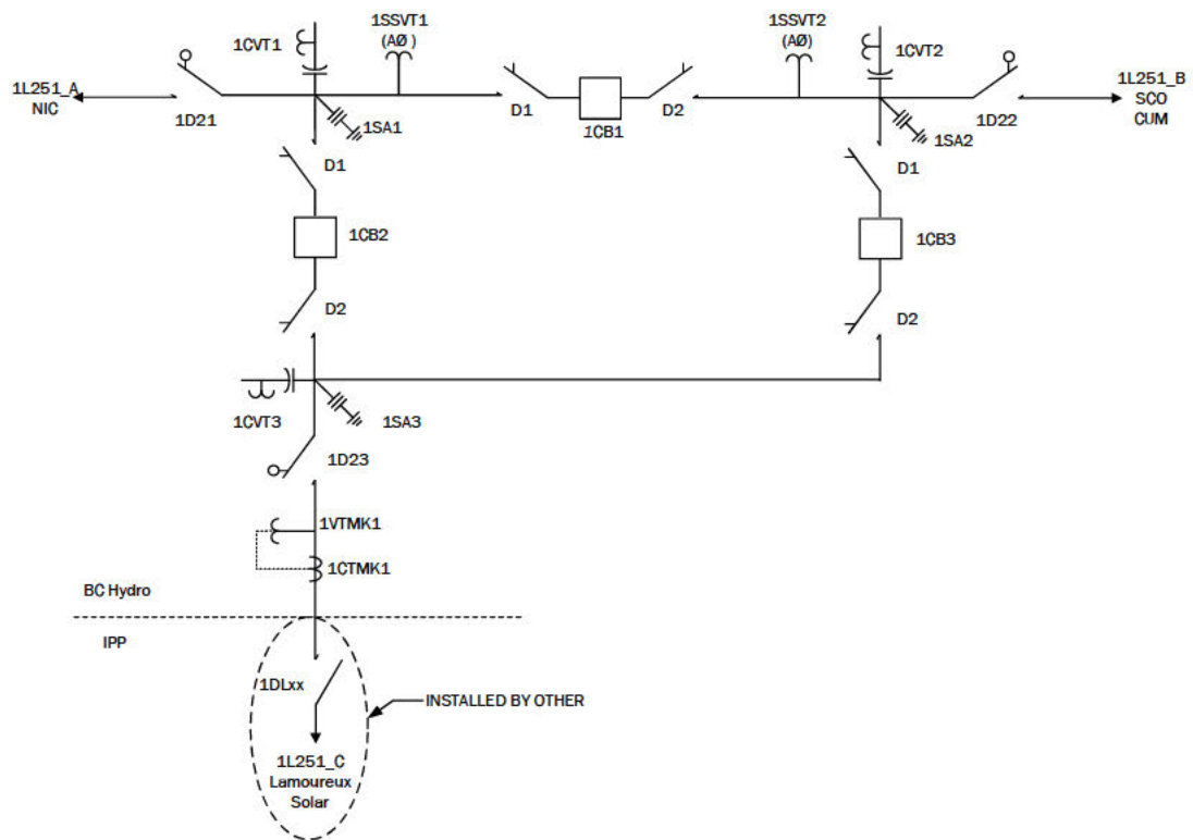
Figure B-1: Stations Planning One-Line Sketch for the New Switching Station P52T.
