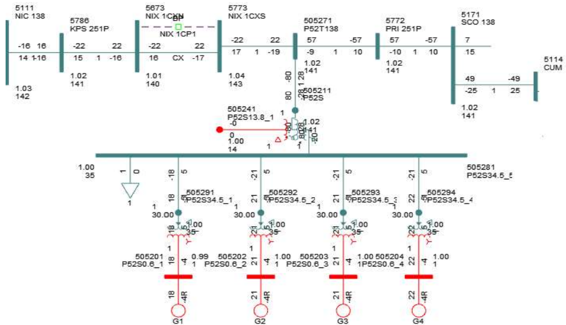
Figure A-1: Lamoureux Project Single Line Diagram for Power Flow Study.
