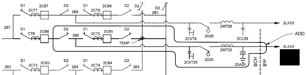
Figure C-1: Stations Planning One-Line Sketch for the Nicola substation upgrade.
