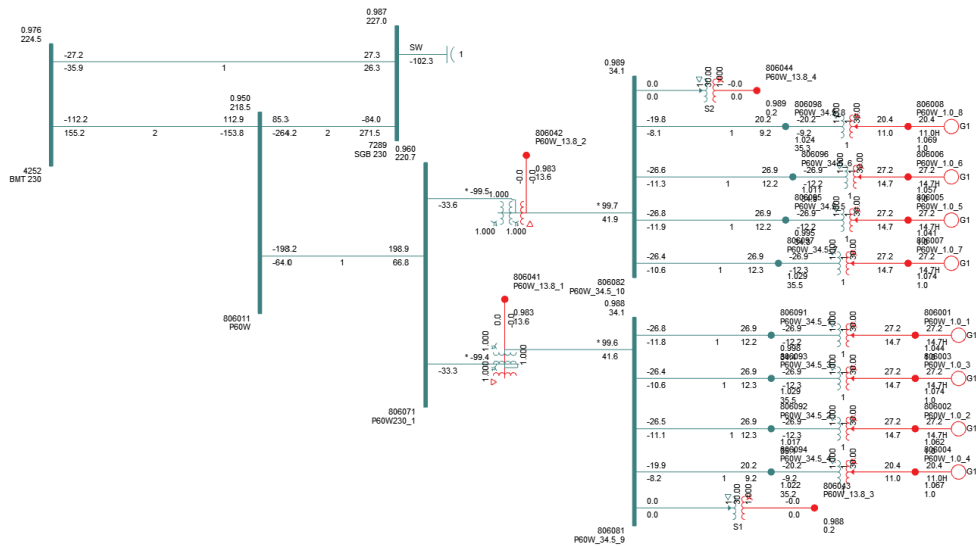
Figure A-1: [redacted] Plant Schematic Diagram.
