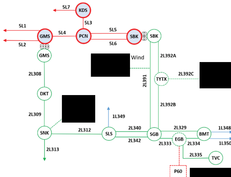
Figure 1-1: Peace Region Transmission System Diagram
