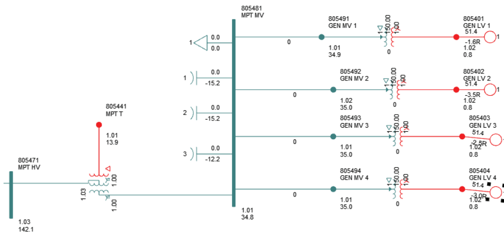
Figure A-1: [REDACTED] Plant Schematic Diagram.
