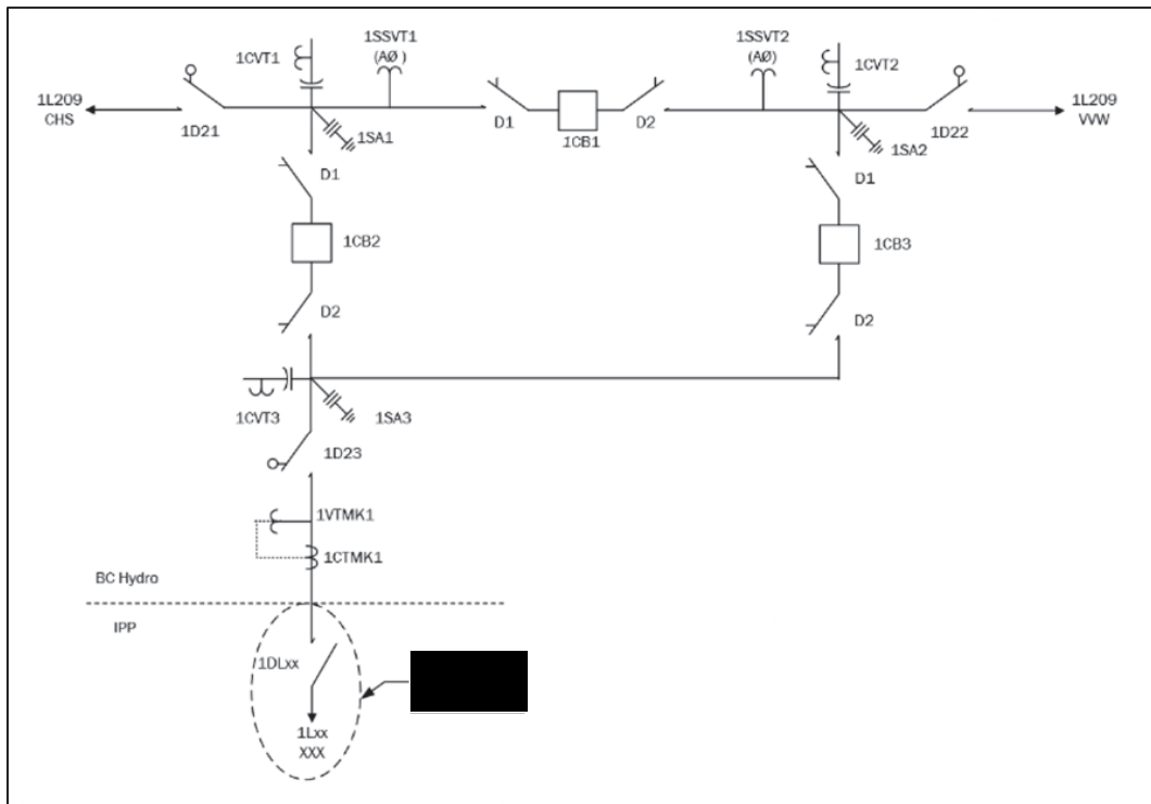
Figure C-1: Stations Planning One-Line Sketch for the New Switching Station P45T.
