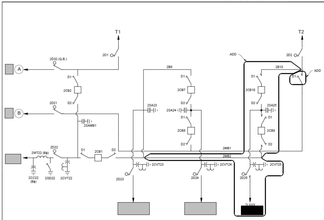
Figure C-1: Stations Planning One-Line Sketch for GLN.
