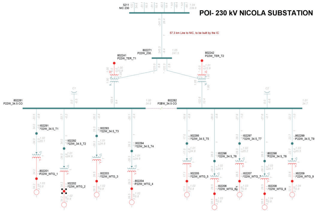
Figure A-1: [REDACTED] Plant Schematic Diagram.
