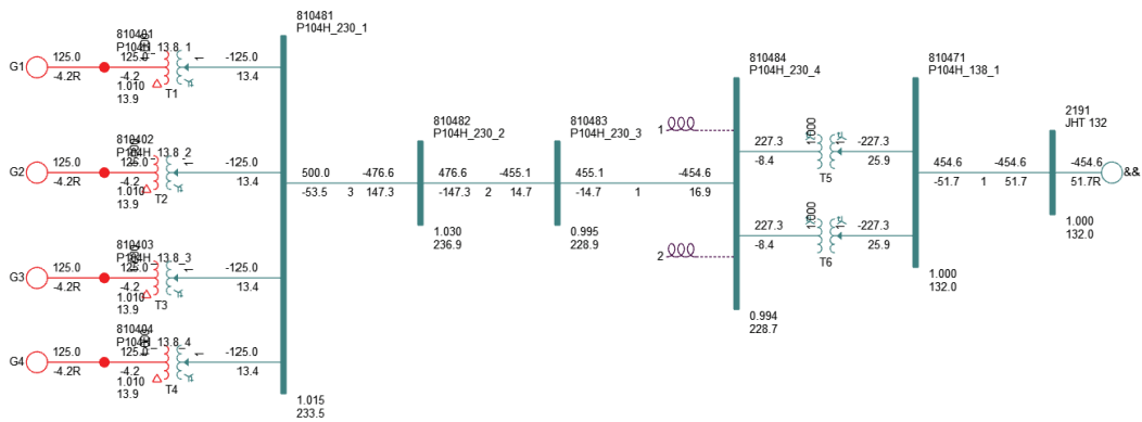
Figure A-1: [REDACTED] Project Plant Schematic Diagram.
