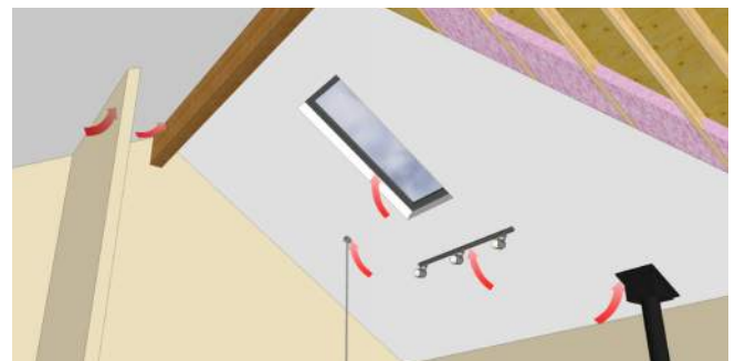
Cathedral ceiling air sealing locations.
